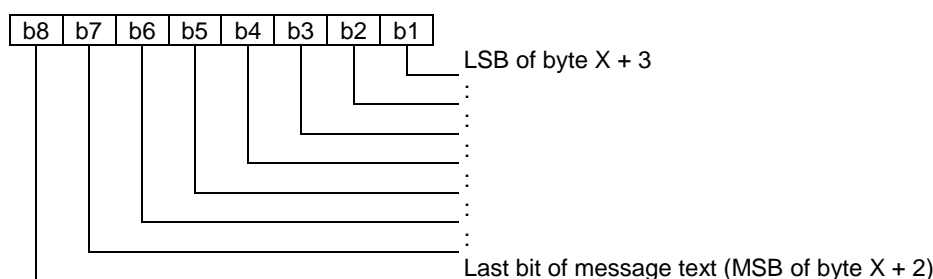
Figure 42: Coding of SDS-1 message text
