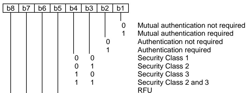
Figure 30: Coding of Security settings
