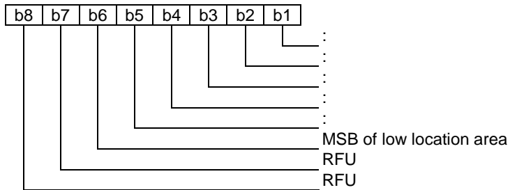
Figure 19: Low location area
