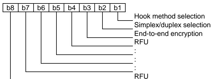
Figure 38: Coding of call modifier bytes 1 and 2
