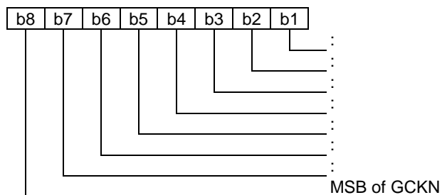
Figure 25: Coding of GCKN
