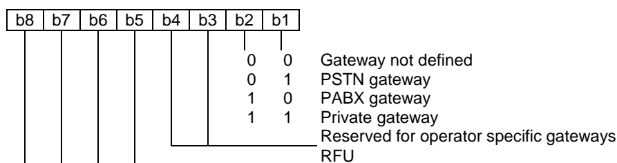
Figure 37: Coding of type of gateway
