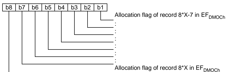
Figure 53: Coding of allocation flags
