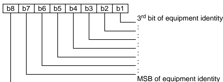
Figure 54: Coding of DMO equipment type and identity
