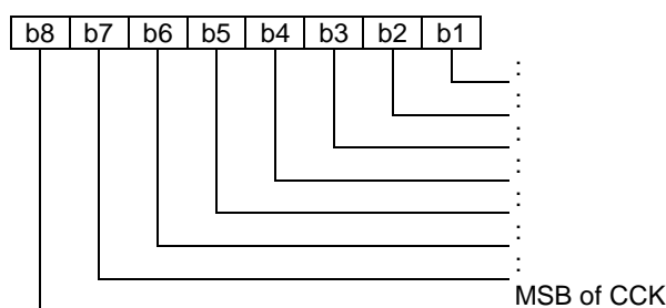
Figure 14: Coding of CCK
