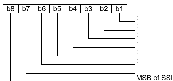
Figure 36: Coding of gateway SSI
