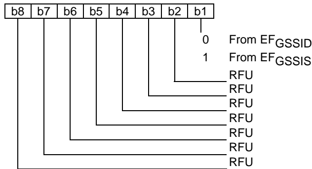
Figure 28: TMO user's preferred group
