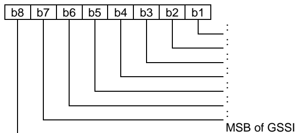
Figure 23: Coding of Group Identity
