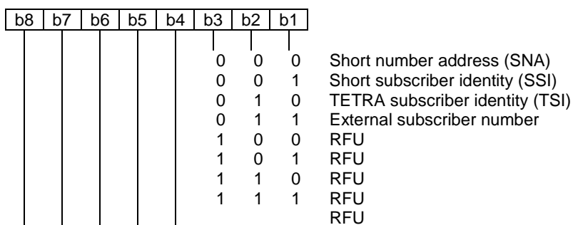
Figure 46: Coding of address type identifier
