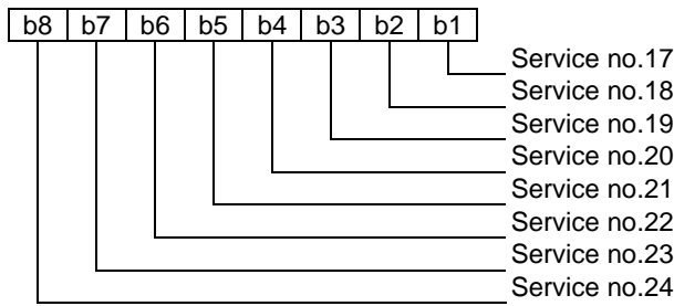
Figure 7: Coding of the SIM service table parameters
