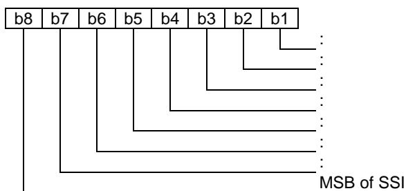
Figure 48: Coding of ITSI/GTSI
