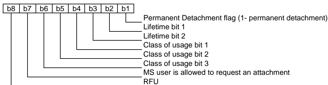
Figure 24: Coding of Group related data
