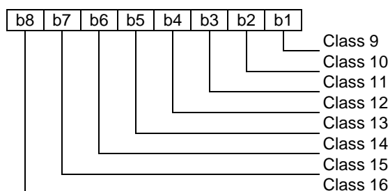
Figure 11: Coding of subscriber classes
