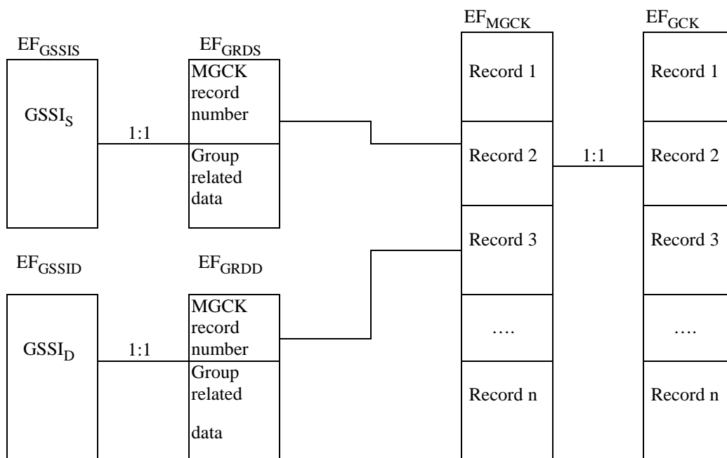
Figure D.1: Graphical presentation of group data related EF structures
