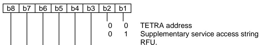
Figure 40: Coding of type
