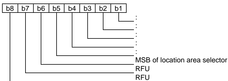
Figure 18: Location area selector
