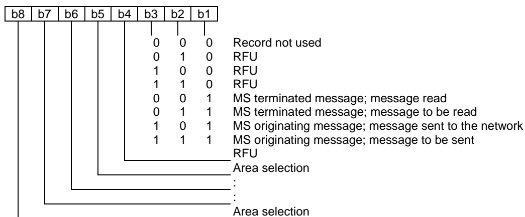
Figure 43: Coding of message status and area selection
