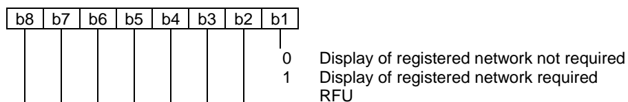
Figure 33: Coding of Display condition
