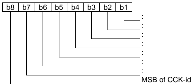
Figure 13: Coding of CCK-id
