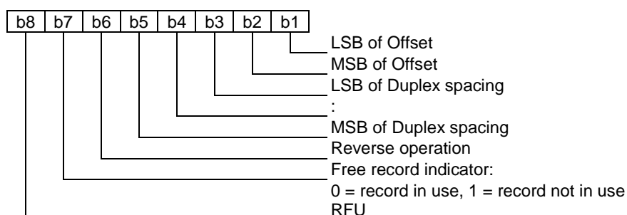
Figure 34: Coding of MCCH information
